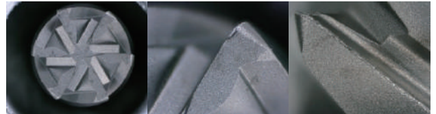
Tool after milling
